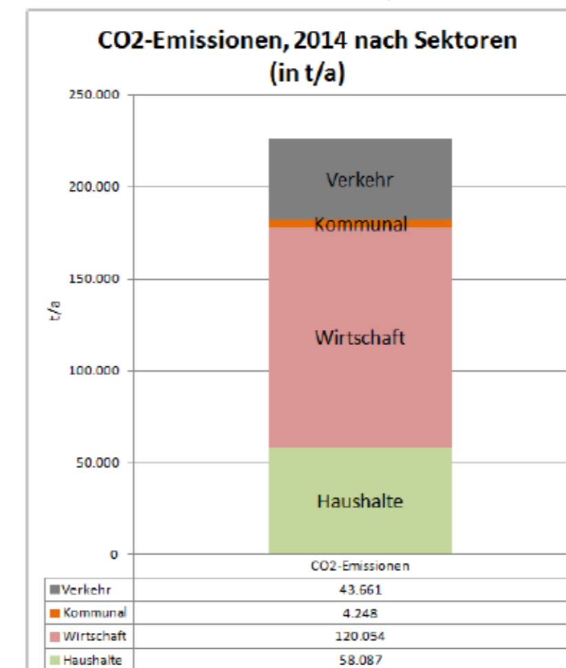
Abb. 28: CO 2 -Bilanz in Reinbek, 2014
